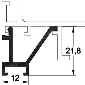
95-741 AĞIRLIK : 0.268 kg/mt
